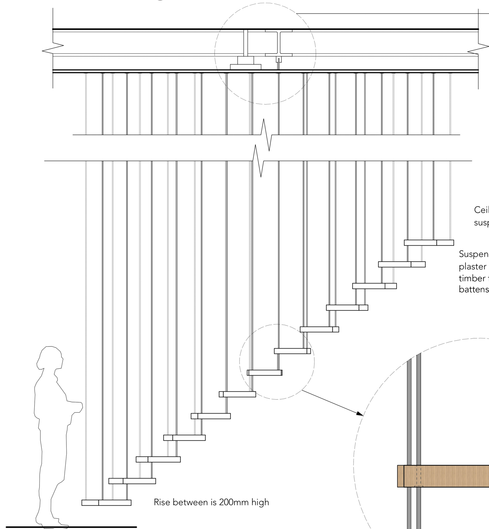
Staircase design Scale @1:20 at A3
